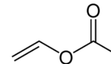
Vinyl Acetate
