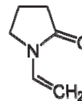
1-Vinyl-2-pyrrolidone
